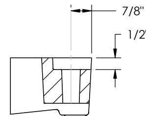
SECTION C-C SCALE 1 : 4
